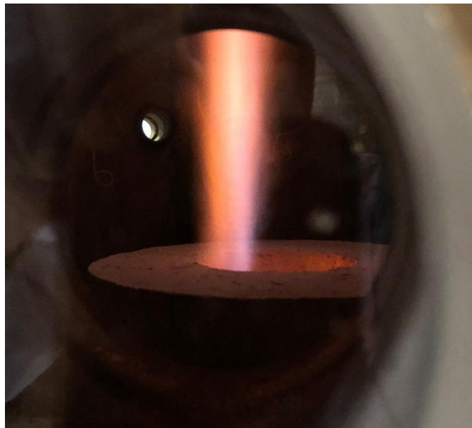
Figure 3 - Air Staged Hydrogen Burner Firing Vertically in a Fluid Heater
