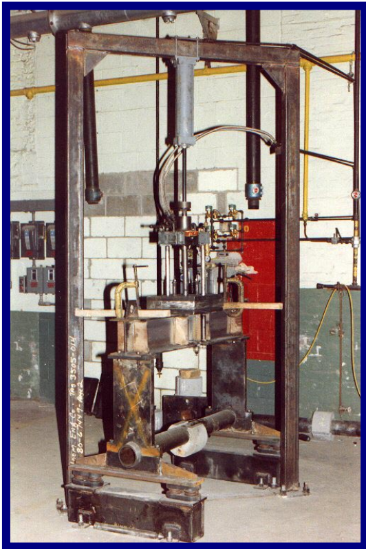
The "Thumper" Machine
